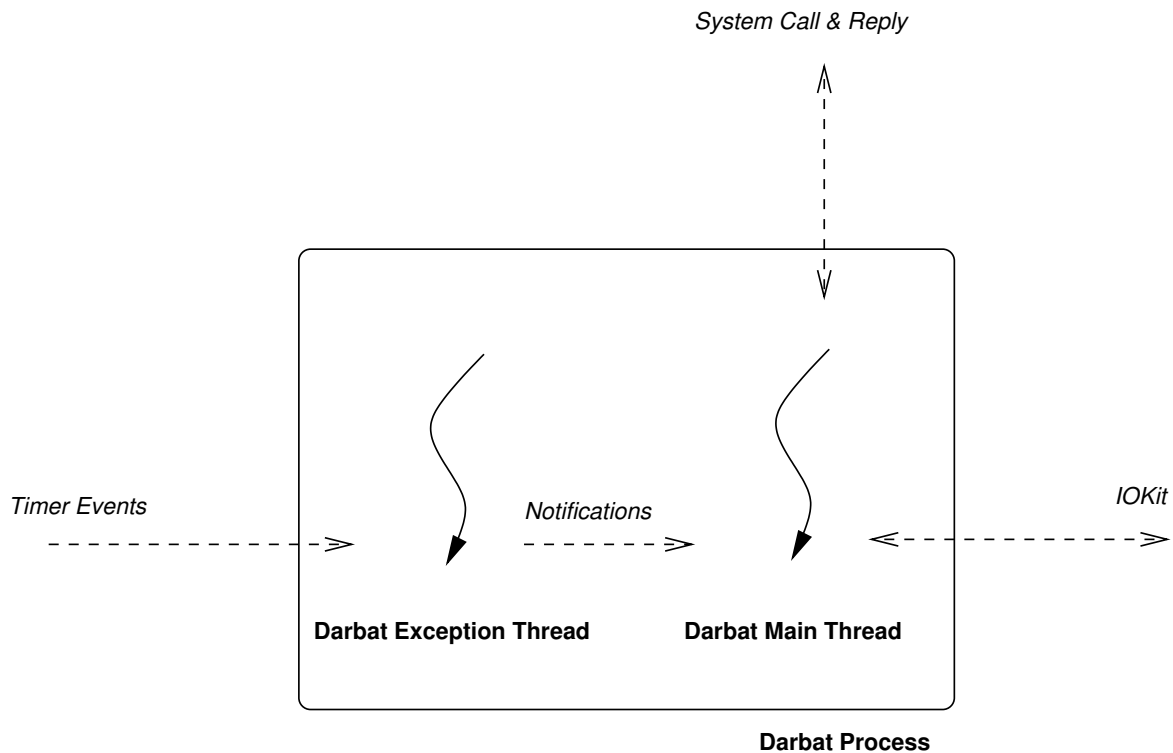
Figure 4.3: Darbat Threading and Messaging
