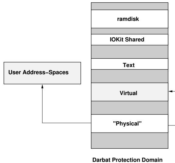
Figure 4.2: Darbat Address Space
