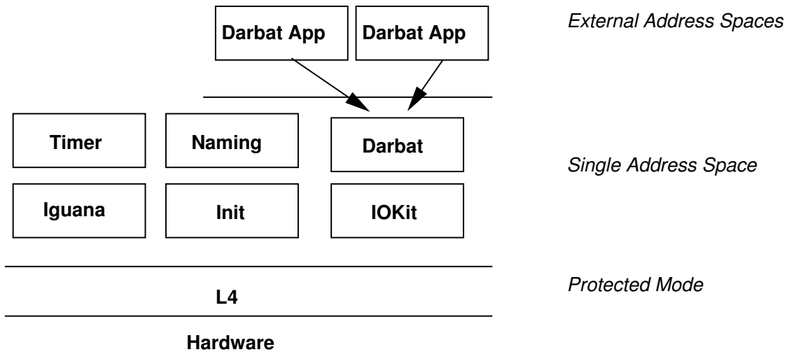
Figure 4.1: Darbat Architecture
